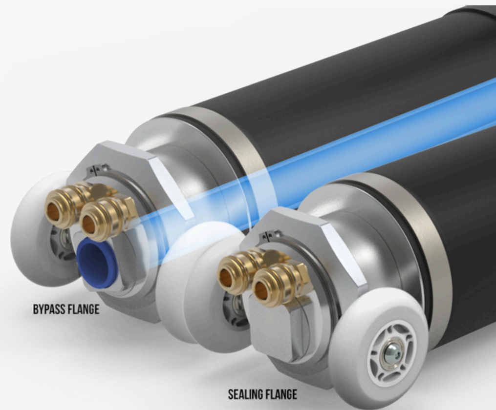
FLOW THROUGH PACKERS
